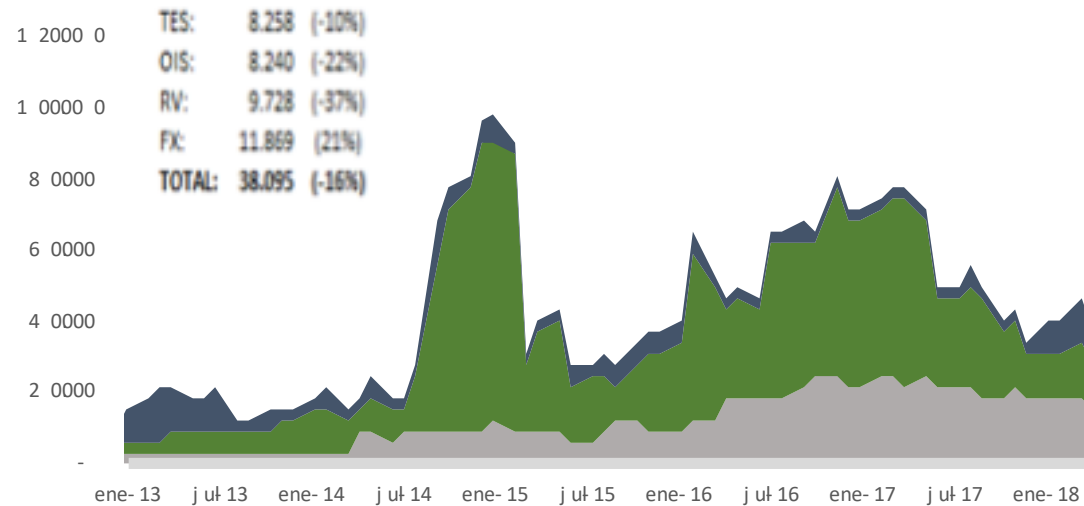
Niveles de Open Interest
